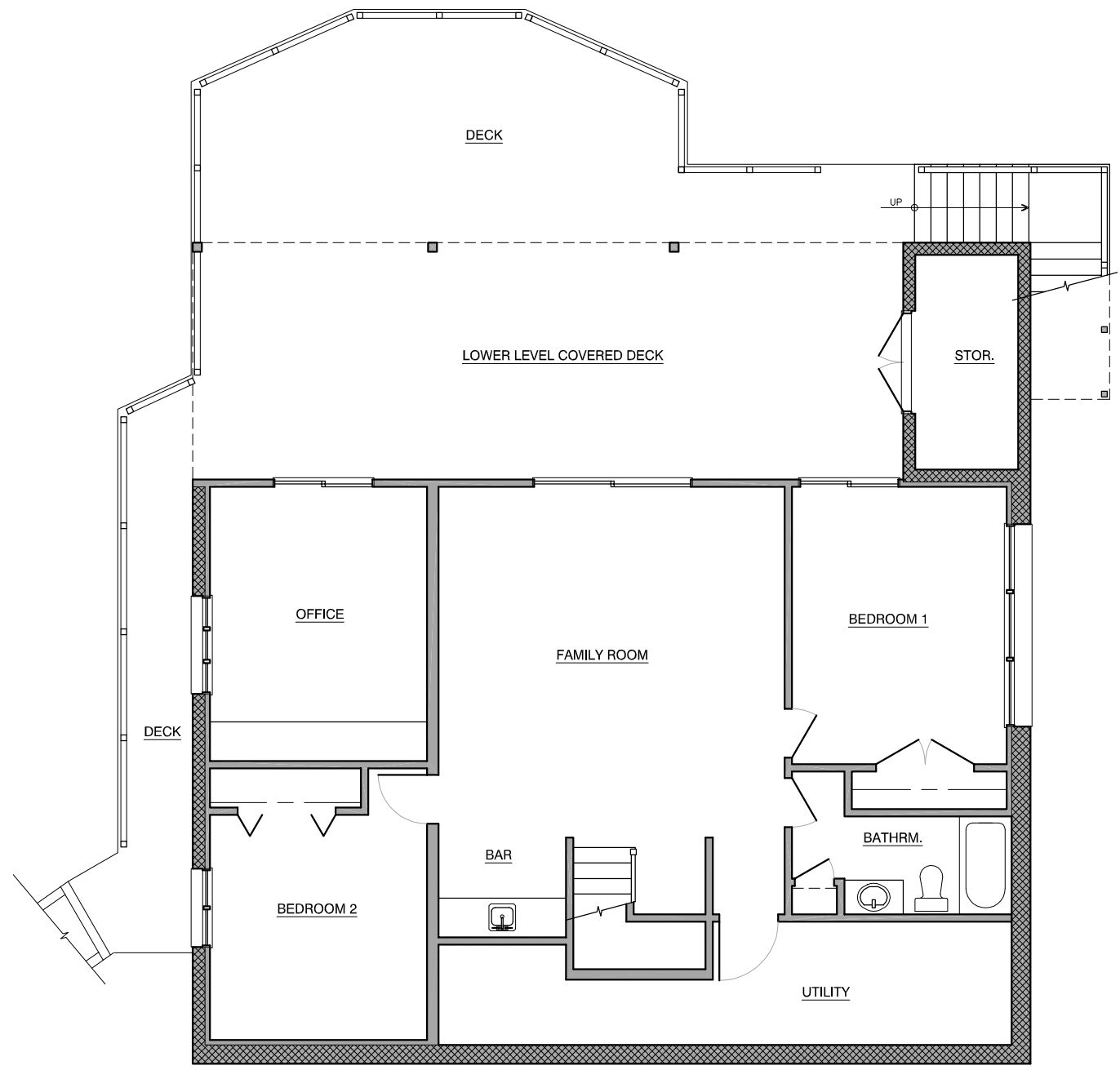
BSMT. LEVEL FLOOR PLAN ARCHITECTURAL
